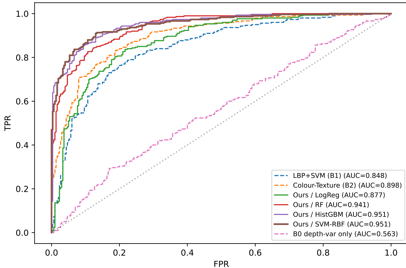
CelebA-Spoof held-out 20% test (n=600)
